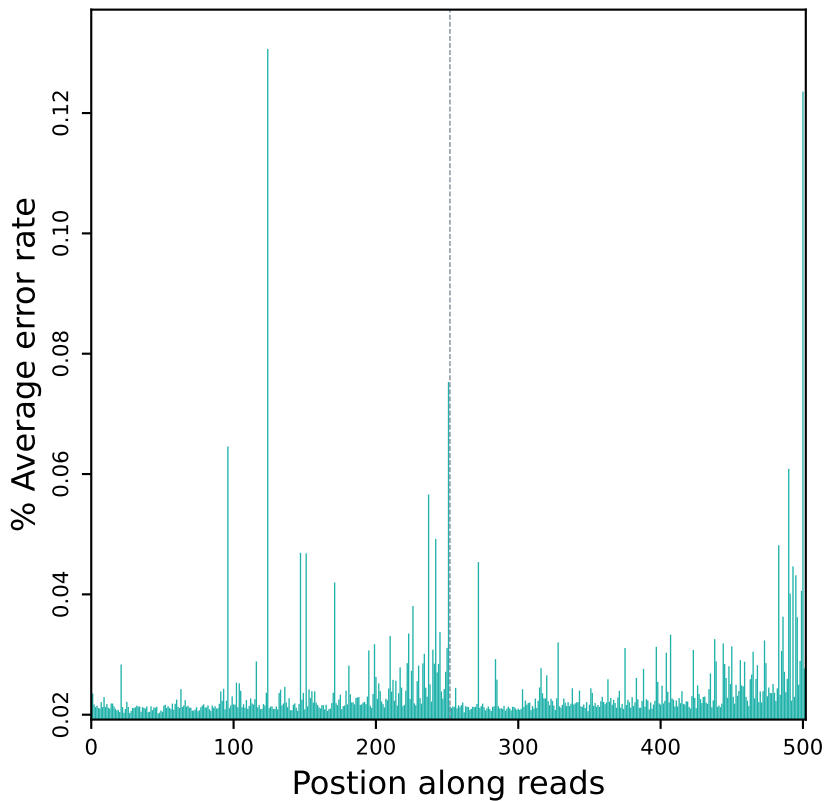
Error rate distribution along reads (R10429)
